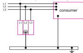
Three phase protection IT system
