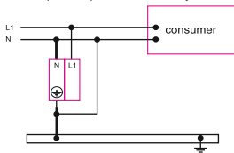
Monophase protection TT system
